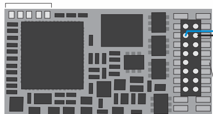
MX645P 16 Top Side (with P1uX16)
