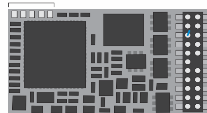
MX645P 22 Top Side (with P1uX22)
