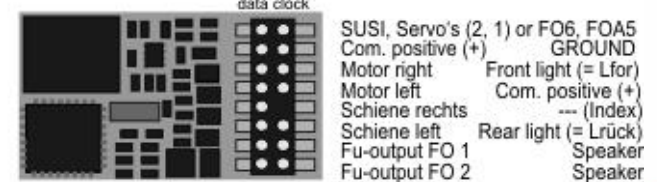
MX648P (with PluX16)
